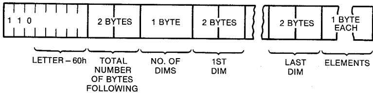
Fig. 3-7. Data structure for string array.
